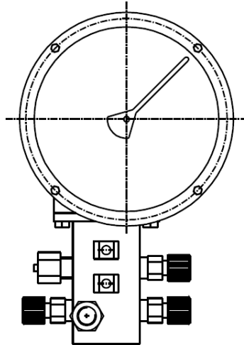
Level indicator and valve block. Pressure gauge not included
